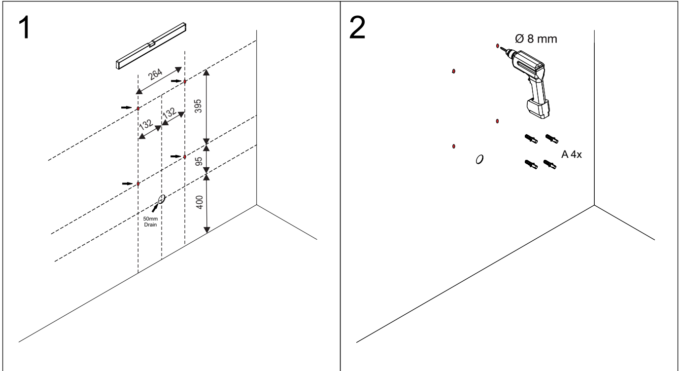
Mark 4 holes for mounting plate
