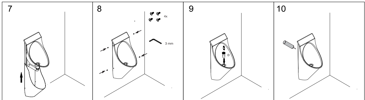
Attach the skirt by gliding it from below into position and align the nuts in FIG. 6
